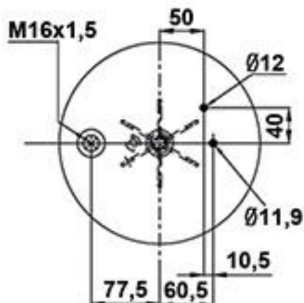
INFERIOR / BOTTOM VIEW
